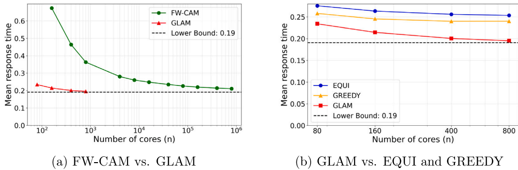
Fig. 3. Performance evaluation of core allocation policies under a representative setting: two classes with sub-linear speedup functions, Poisson arrivals, and Exponential job sizes, with system load fixed at \rho = 0.6 as n scales. The same qualitative behavior is observed across all other settings we tested; see Appendix K for additional inter-arrival time and job size distributions and for full workload details.
