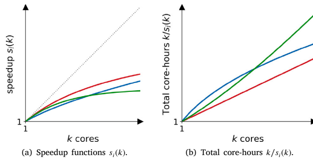
Fig. 1. Examples of speedup functions and the corresponding total core-hours (assuming job size is 1). Speedup functions are typically sublinear and concave; k/s_i(k) is increasing and at least 1, but it is not restricted to being convex or concave.
